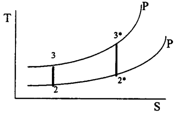
Figure 2: Compression T-S Diagram
